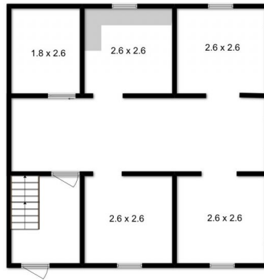
Shed 8.0 x 8.0
