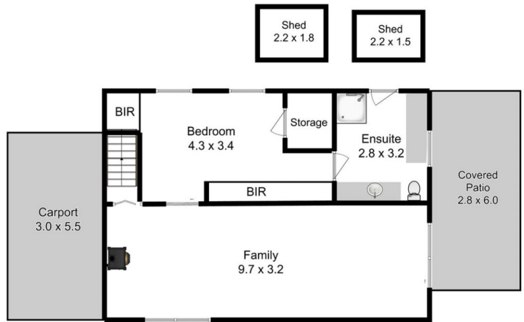
Lower Level
